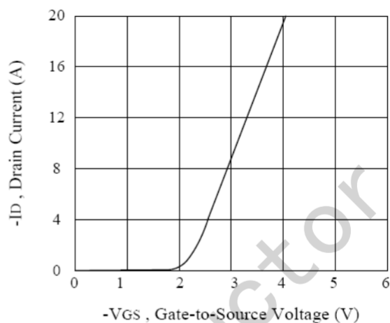
Figure 12. Transfer Characteristics
