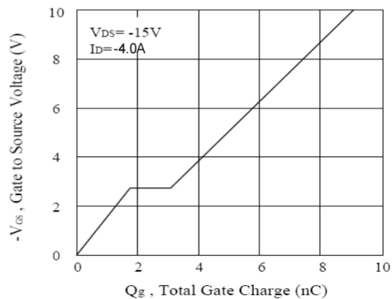
Figure 15. Gate Charge
