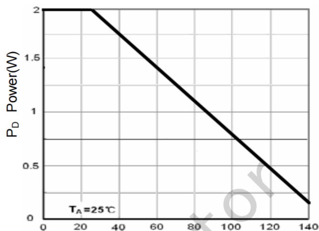
T_J -Junction Temperature( ^\circ C ) Figure 8 Power Dissipation
