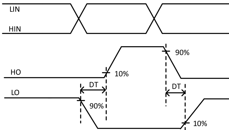
Figure Cross Conduction Prevention Delay Time Waveform Definition
