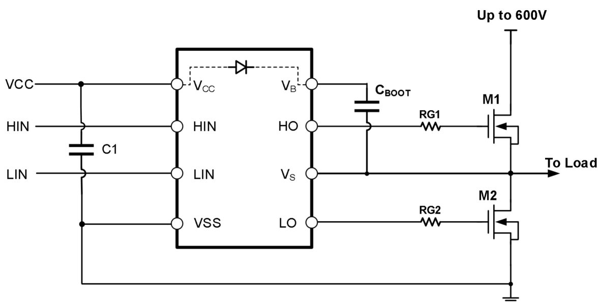
Figure Typical application circuit of UCC27710
