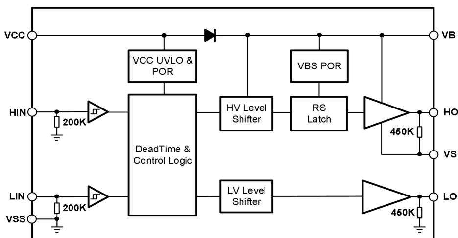
Figure Function Block Diagram of UCC27710
