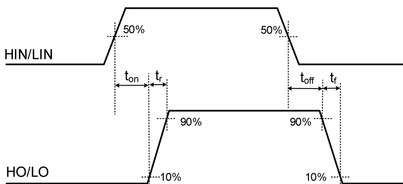
Figure Propagation Time Waveform Definition
