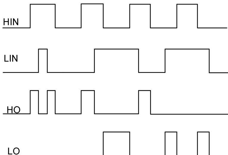
Figure UCC27710 Input and output timing waveform
