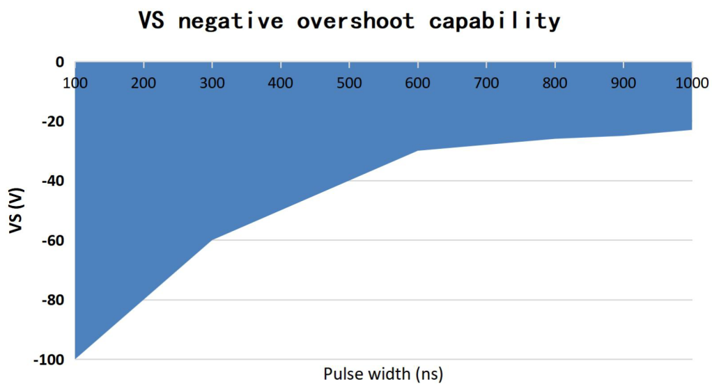
Figure The relationship between VS negative overshoot and duration
