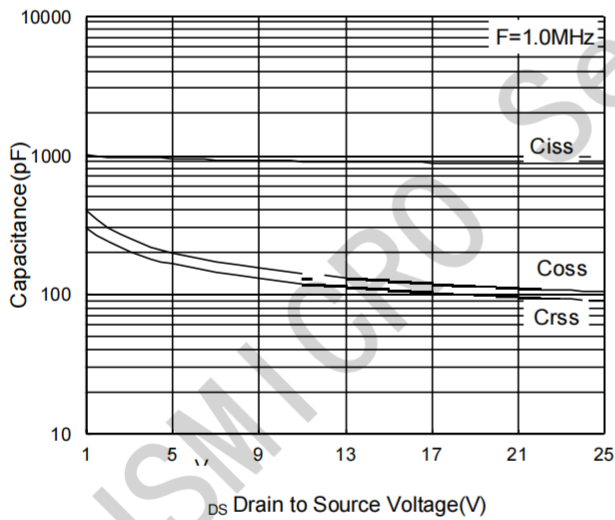
Fig.7 Capacitance
