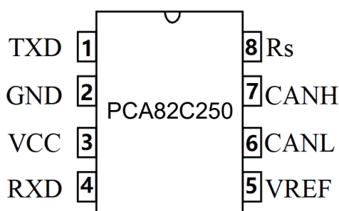
SOP-8/MSOP-8
