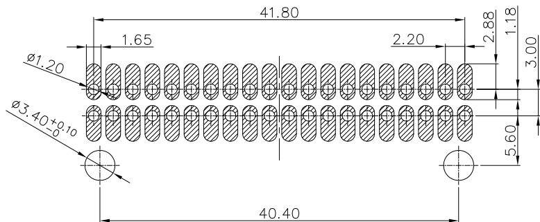
RECOMMENDED PCB LAYOUT (TOP SIDE) TOLERANCE \pm 0.05
