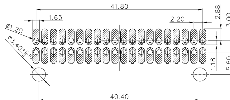
RECOMMENDED PCB LAYOUT (BOTTOM SIDE) TOLERANCE \pm 0.05
