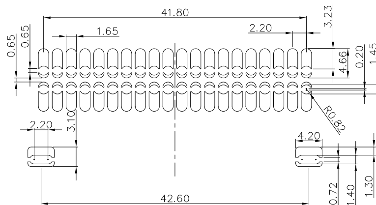
STEEL MESH (BOTTOM SIDE) T \geq 0.12\text{mm}
