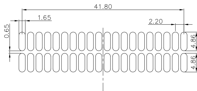
STEEL MESH (TOP SIDE) T \geq 0.12\text{mm}
