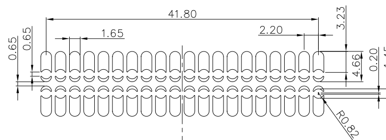
STEEL MESH (BOTTOM SIDE) T \geq 0.12\text{mm}
