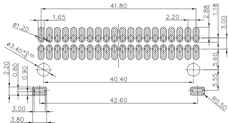
RECOMMENDED PCB LAYOUT (TOP SIDE) TOLERANCE \pm 0.05
