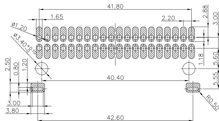
RECOMMENDED PCB LAYOUT (BOTTOM SIDE) TOLERANCE \pm 0.05
