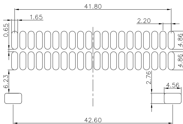
STEEL MESH (TOP SIDE) T \geq 0.12\text{mm}
