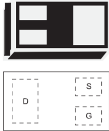
DFN1006-3L
