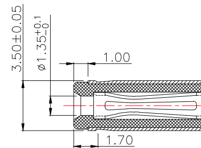
MATING PLUG
