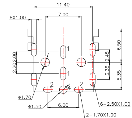
RECOMMENDED PCB LAYOUT GENERAL TOLERANCE \pm 0.05
