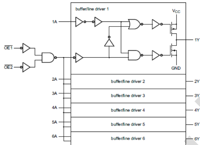
Figure 4. Logic diagram
