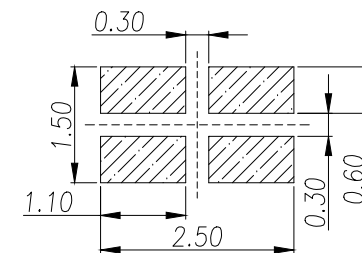
METAL MASK T=0.08
