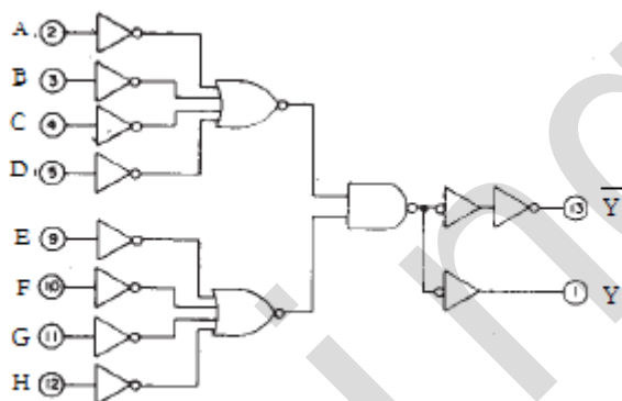
Figure 2. Logic diagram
