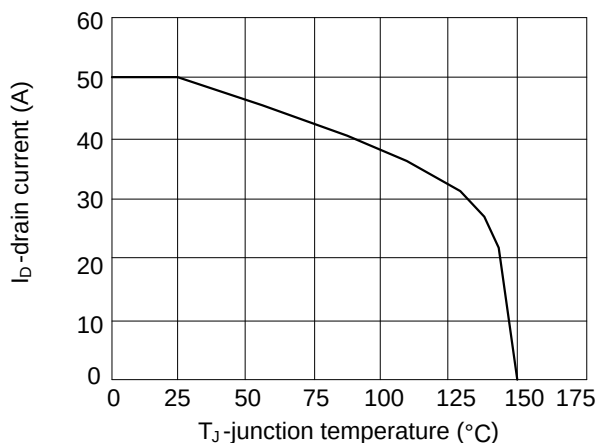
Figure 10 Current de-rating
