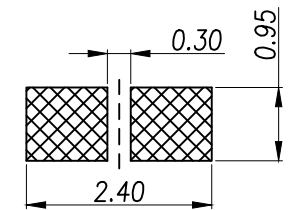
METAL MASK T=0.08
