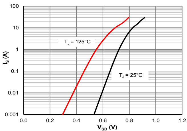
Figure 5: Body-Diode Characteristics
