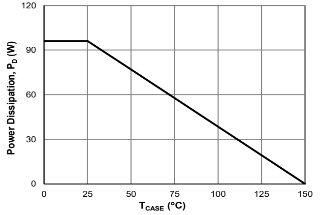
Figure 8: Power De-rating
