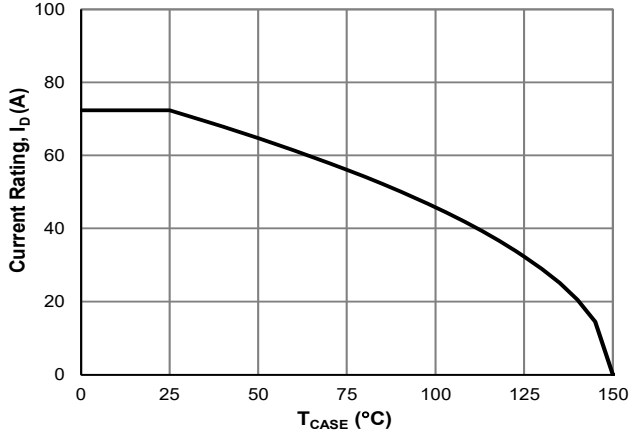
Figure 7: Current De-rating
