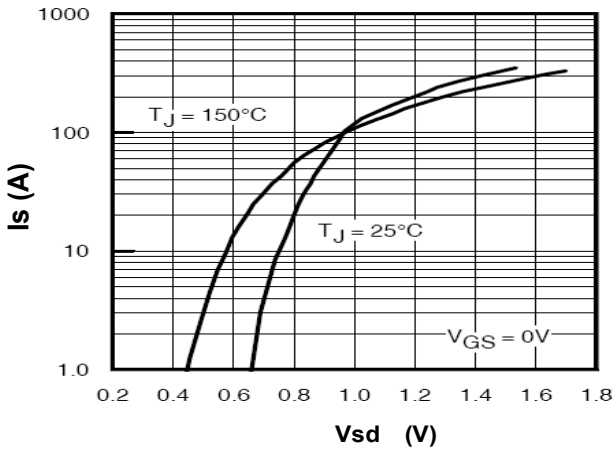
Figure 9. Body-Diode Characteristics
