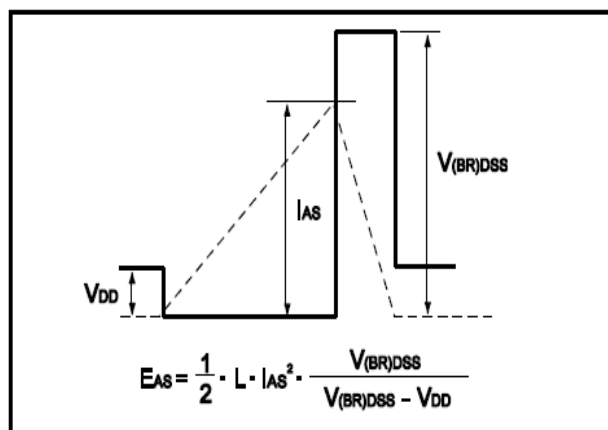
Fig.12 Avalanche Waveform
