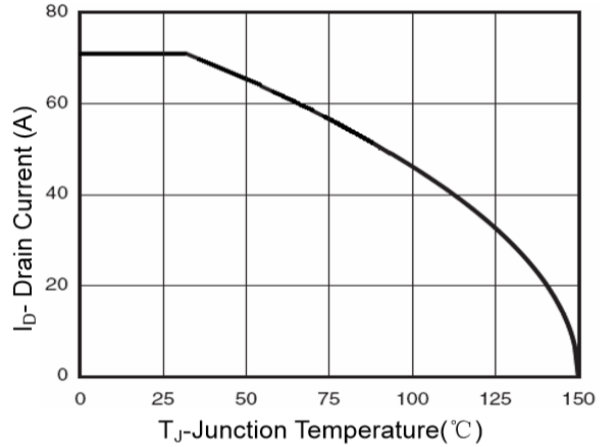
Figure 10 I_D Current Derating vs Junction Temperature
