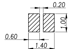
METAL MASK T=0.10 TOLERANCE ±0.05 (角公差)
