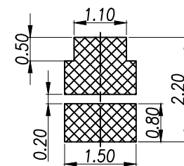
METAL MASK T=0.08
