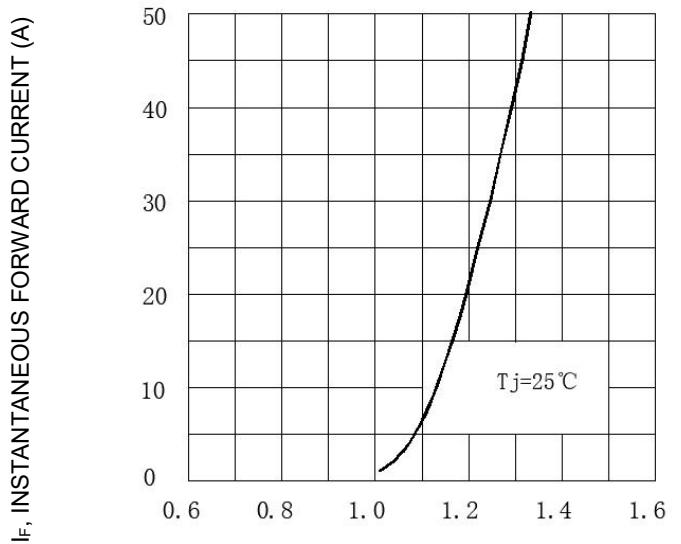
Fig.2 Maximum Forward Characteristics, per element
