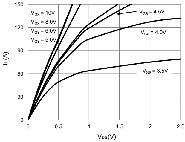
Figure 1: Saturation characteristics
