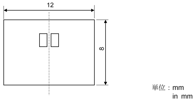
Figure 5. Test Board for Bending Strength Test
