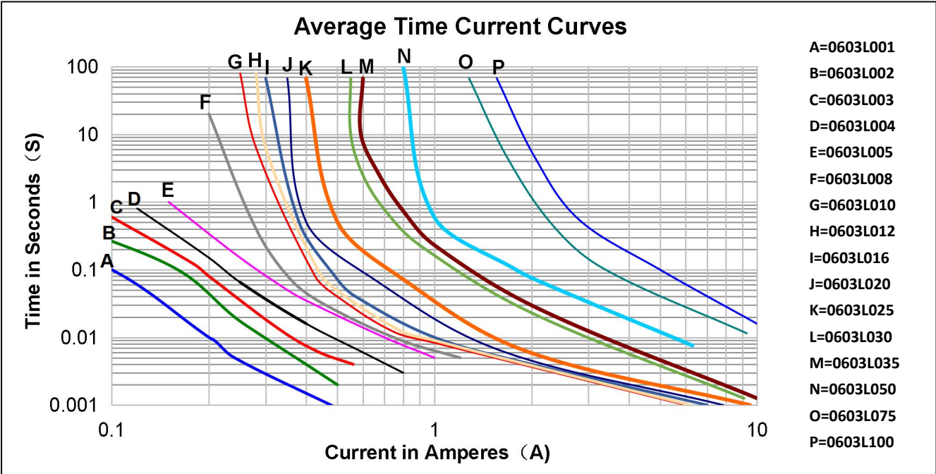
Typical Time-to-Trip at 25°C/25°C跳闸保护时间曲线表
