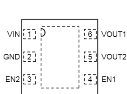
6-Pin 1.6mm x 1.6mm Thin MLF (MT) / MLF (ML) Top View
