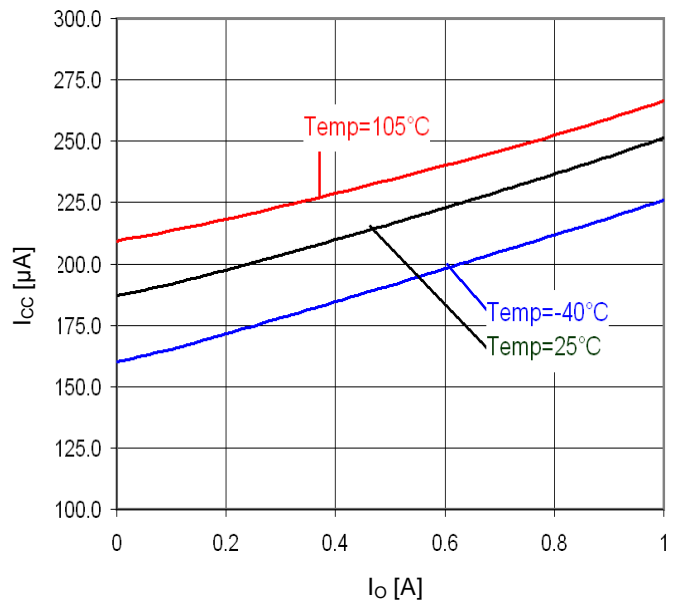
Figure 32. I_o - I_{cc}
