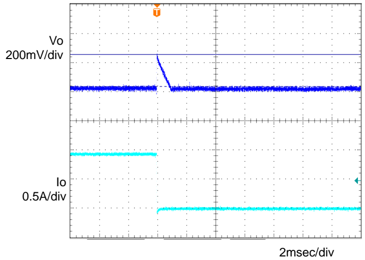
Figure 6. Transient Response (1.0→0A) Co=1\mu F, Ta=-40^{\circ}C
