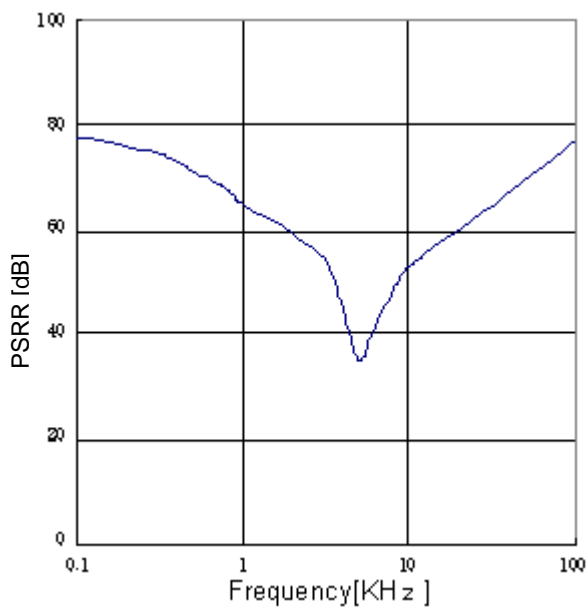
Figure 33. PSRR ( I_o=0\text{mA} )
