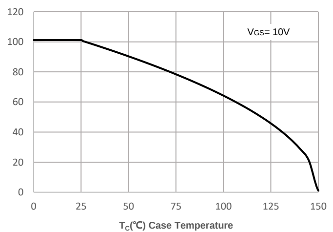
Figure 10: Maximum Continuous Driant Current vs. Case Temperature
