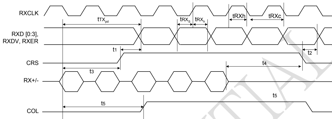
9.4.10 MII 100BASE-TX Receive Timing Diagram
