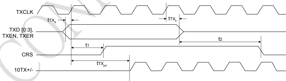
9.4.12 MII 10BASE-T Nibble Transmit Timing Diagram
