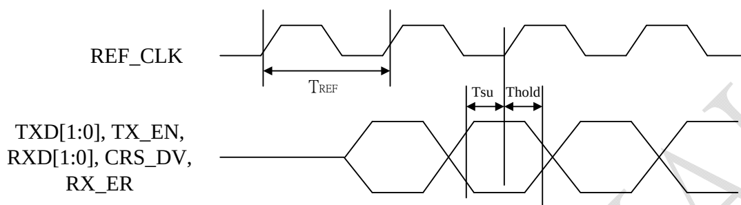
9.4.19 RMII Timing Diagram
