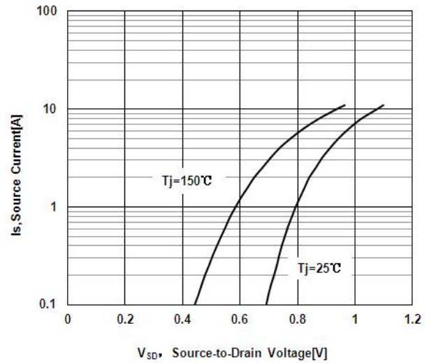
Figure 4. Body-Diode Characteristics
