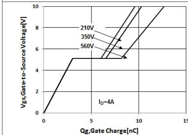
Figure 5. Gate-Charge Characteristics
