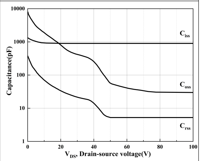
Figure 4. Typical Capacitance
