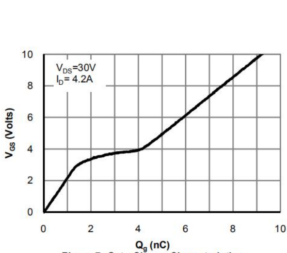
Figure 7: Gate-Charge Characteristics
