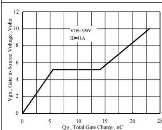
Figure 5. Gate-Charge Characteristics
