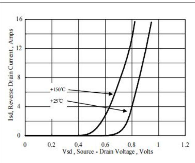
Figure 4. Body-Diode Characteristics
