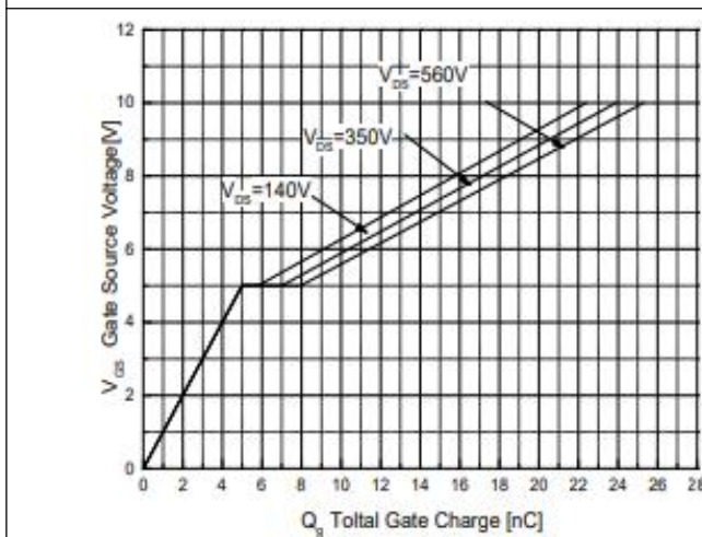
Figure 5. Gate-Charge Characteristics
