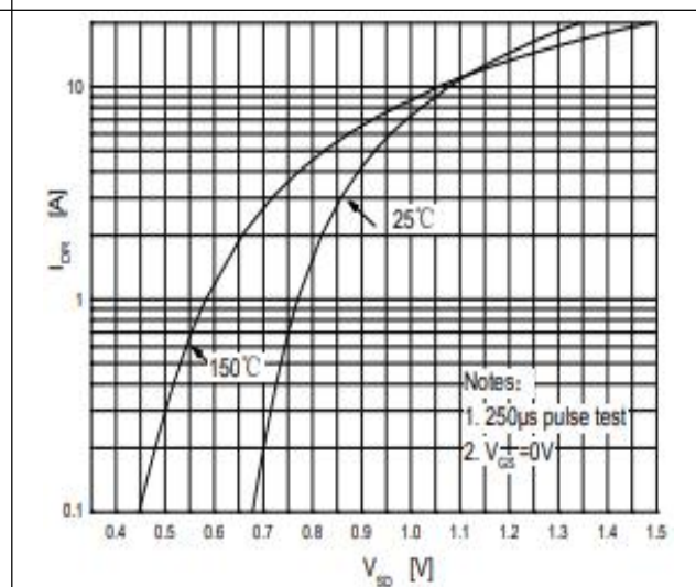
Figure 4. Body-Diode Characteristics
