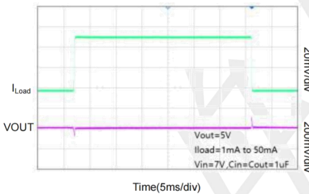
Load-Transient Response
