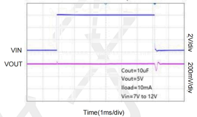
Line-Transient Response
