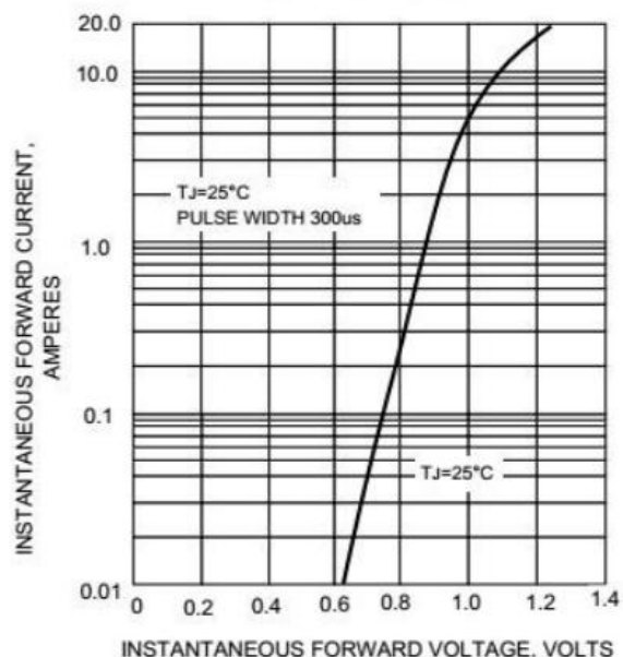
FIG.3-TYPICAL FORWARD CHARACTERISTICS
