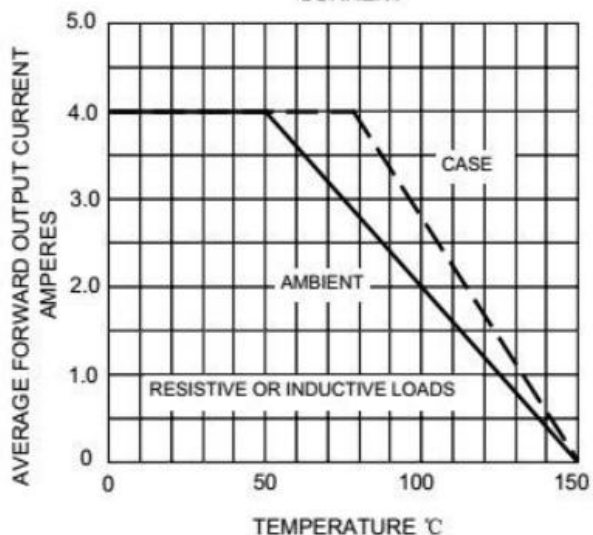
FIG.2-FORWARD DERATING CURRENT
