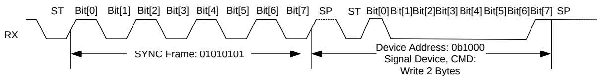
Figure 12: Synchronization Byte
