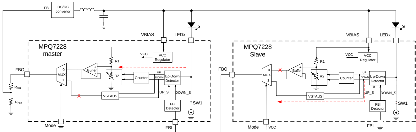
Figure 4: Master and Slave Mode Set-Up
