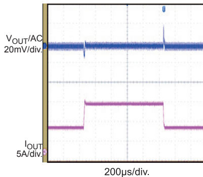
Load Transient
