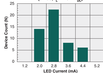
Form-A Typical I_F for Switch Dropout (N=50, I_L=120\text{mA}_{\text{DC}} )
