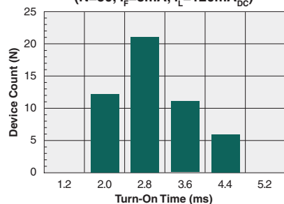
Form-A Typical Turn-On Time (N=50, I_F=8\text{mA} , I_L=120\text{mA}_{\text{DC}} )
