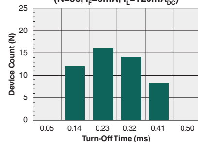
Form-A Typical Turn-Off Time (N=50, I_F=8\text{mA} , I_L=120\text{mA}_{\text{DC}} )
