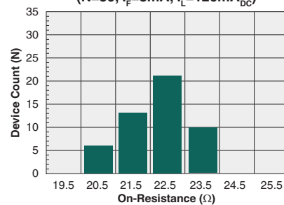
Form-A Typical On-Resistance Distribution (N=50, I_F=8\text{mA} , I_L=120\text{mA}_{\text{DC}} )
