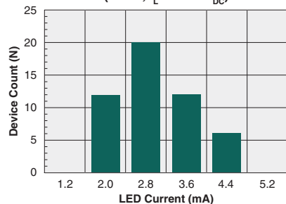
Form-A Typical I_F for Switch Operation (N=50, I_L=120\text{mA}_{\text{DC}} )
