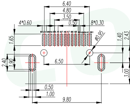
RECOMMENDED P.C.B. LAYOUT (T:1.0~1.2mm) TOLERANCE UNSPECIFIED ±0.05mm
