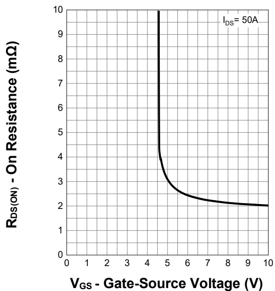
On-resistance gate source voltage
