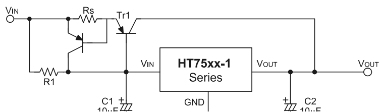
Short-Circuit Protection for Tr1
