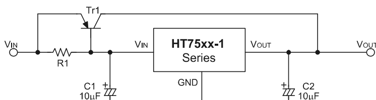
High Output Current Positive Voltage Regulator
