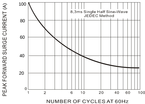
FIG.3 MAXIMUM NON-REPEITIVE SURGE CURRENT
