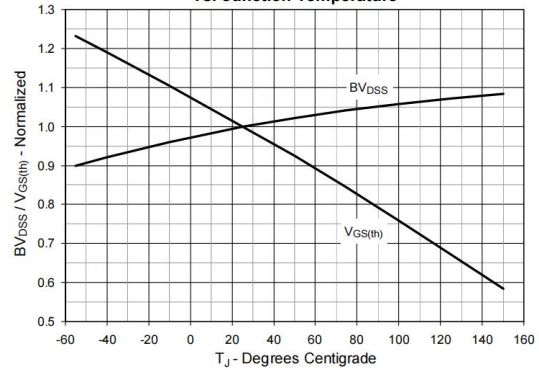
Fig. 6. Normalized Breakdown & Threshold Voltages vs. Junction Temperature
