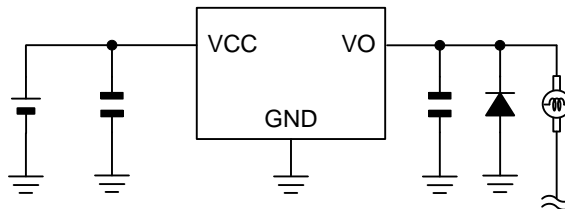
Figure 27. Application Example 3
