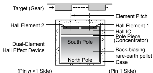
Figure 2. Relative motion of the target is detected by the dual Hall elements mounted on the Hall IC.
