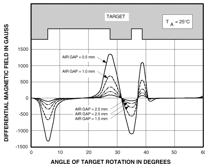
Figure 4. Effect of varying air gaps on differential circuits.
