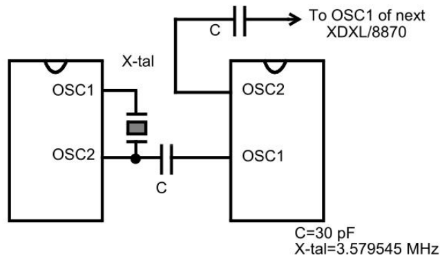
Figure 7 - Oscillator Connection
