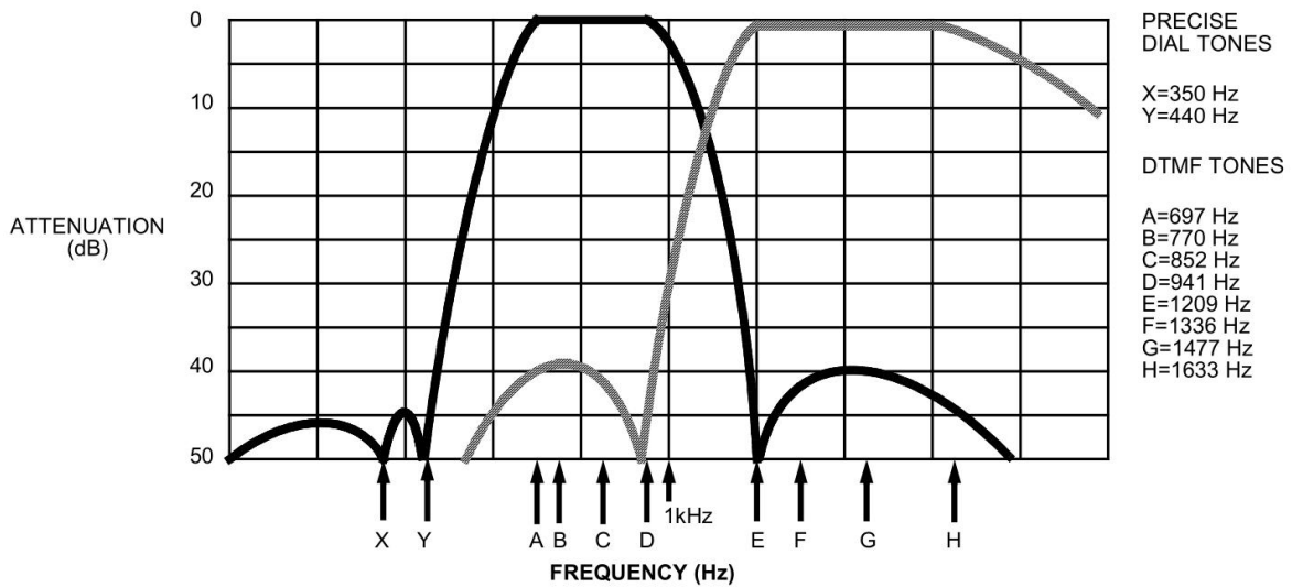
Figure 3 - Filter Response
