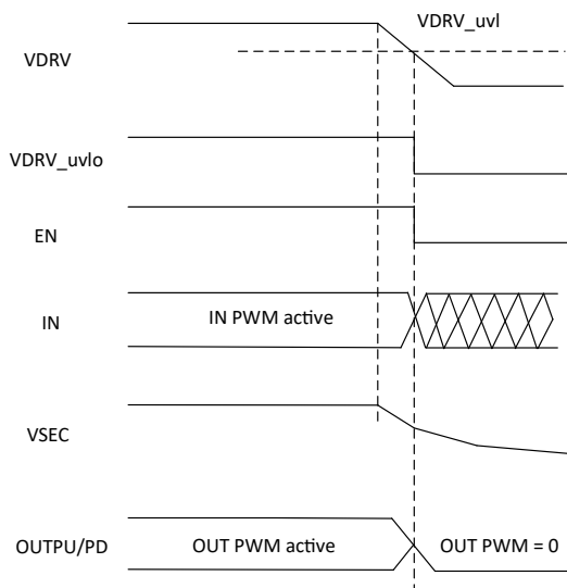
Figure 5: Shutdown Mechanism
