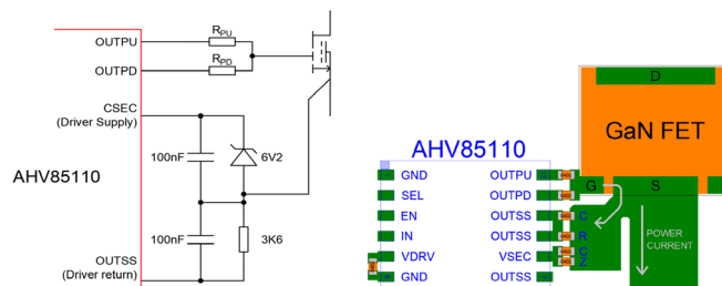
Figure 10: AHV85110 bipolar drive and recommended PCB layout
