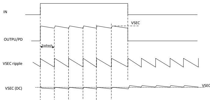
Figure 6: AHV85110 Refresh Mechanism
