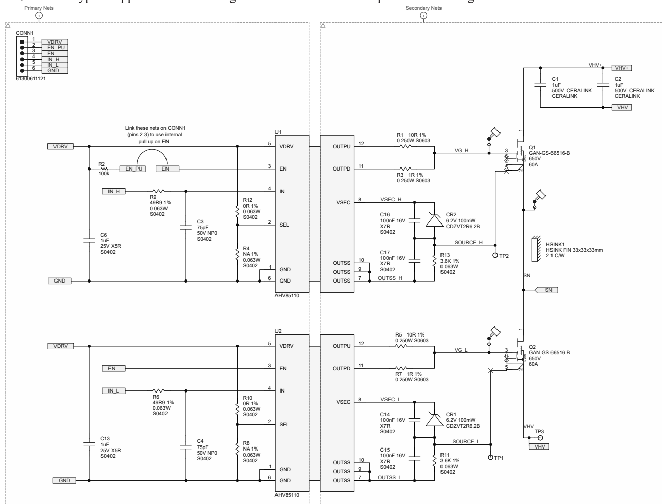
Figure 16: APEK85110KNH-01-T-MH schematic for driving a GaN transistor with a bipolar drive arrangement.
