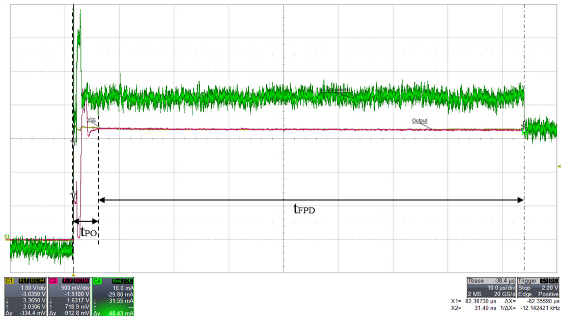
Figure 5: Power-On Behavior
