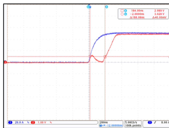
Figure 10: CT430 Propagation Delay; I_P = 50 \text{ A}_{PK} and C_L = 100 \text{ pF} (Blue = I_{CCC} , Red = V_{OUT} )
