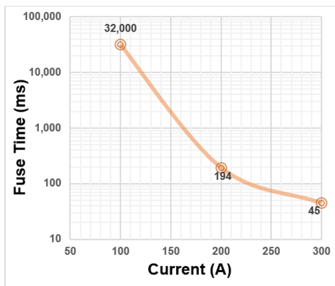
Figure 25: CT430 Fuse Time vs. Current
