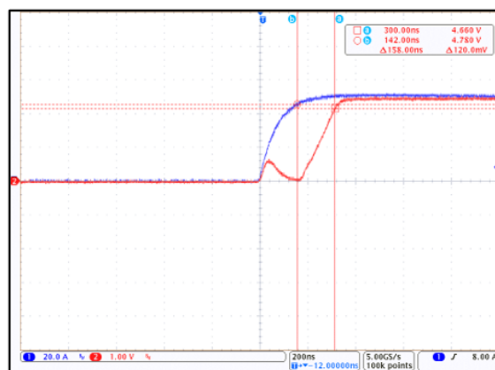
Figure 8: CT430 Response Time; I_P = 50 \text{ A}_{PK} and C_L = 100 \text{ pF} (Blue = I_{CCC} , Red = V_{OUT} )
