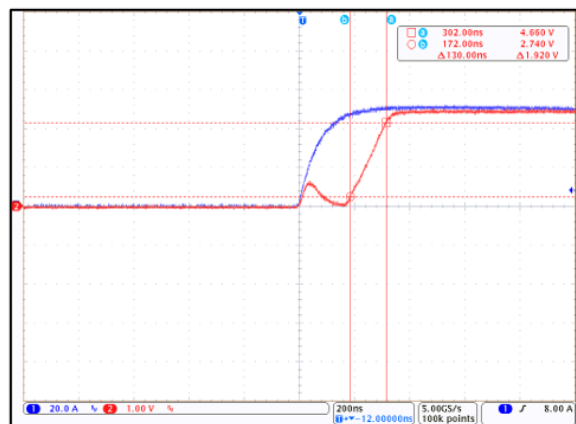
Figure 9: CT430 Rise Time; I_P = 50 \text{ A}_{PK} and C_L = 100 \text{ pF} (Blue = I_{CCC} , Red = V_{OUT} )
