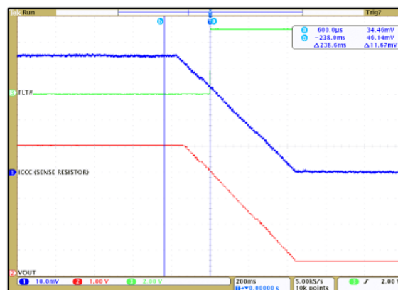
Figure 12: CT430 OCD disabled at 90% of 50\text{ A}_{DC} and \overline{\text{FLT}} is High
