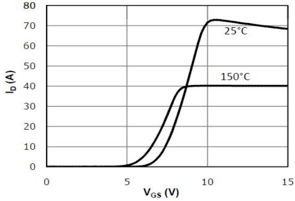
Fig 3: Transfer Characteristics
