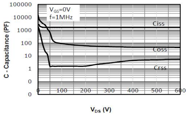
Fig 11: Capacitance Characteristics
