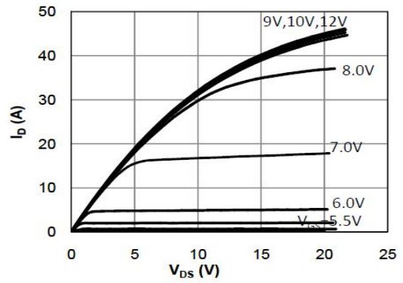
Fig 2. Output Characteristics ( T_j=150^\circ\text{C} )
